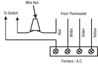
Figure 3: Wiring Diagram for Unit Shutdown
