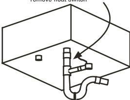
Figure 1: Vertical Drain Outlet Installation
