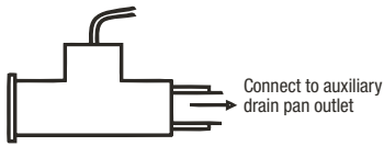
Figure 1: Horizontal (plugged) installation for auxiliary drain outlets.
