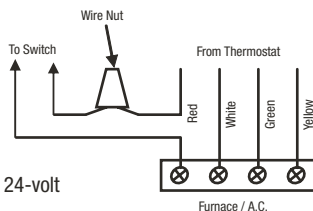
Figure 5: Wiring Diagram for Unit Shutdown
